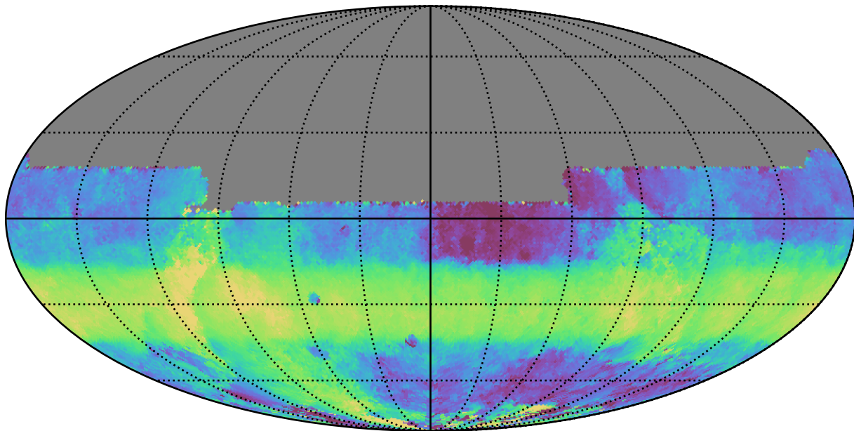
roll_pause_mjdp60_v3.4_10yrs All sky y band: Median HA
