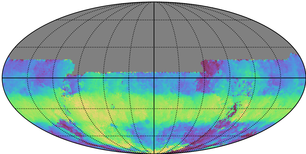
roll_pause_mjdp60_v3.4_10yrs All sky u band: Median HA
