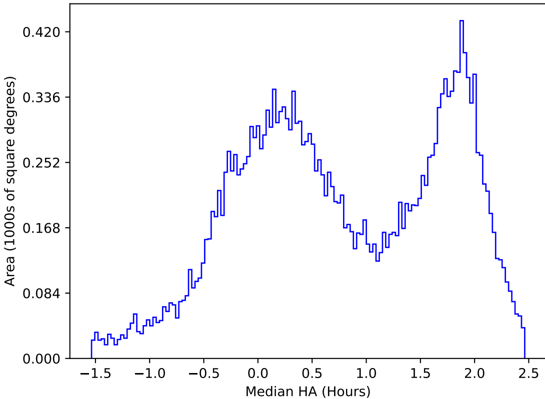
roll_pause_mjdp60_v3.4_10yrs All sky u band: Median HA
