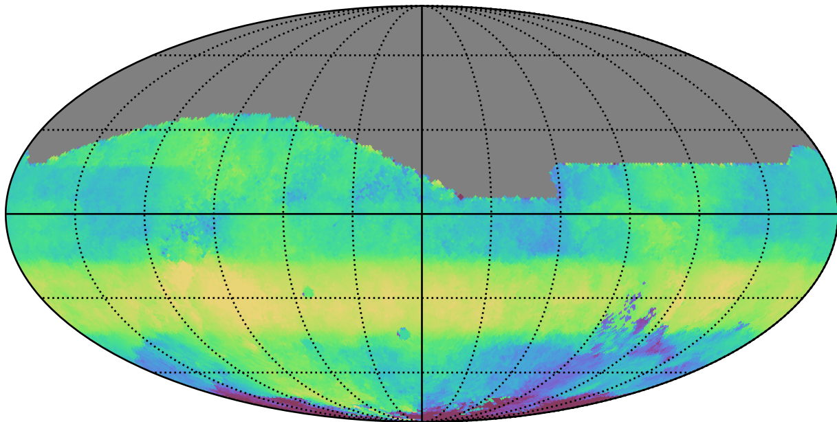
roll_pause_mjdp60_v3.4_10yrs All sky r band: Median HA
