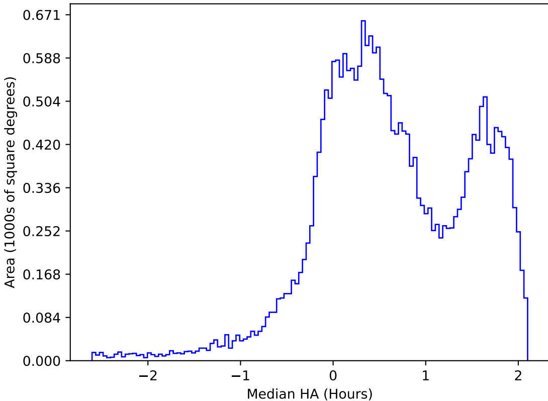
roll_pause_mjdp60_v3.4_10yrs All sky r band: Median HA
