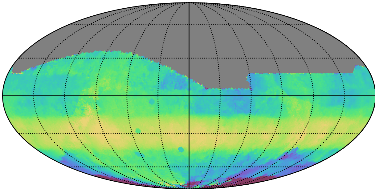
roll_pause_mjdp60_v3.4_10yrs All sky i band: Median HA
