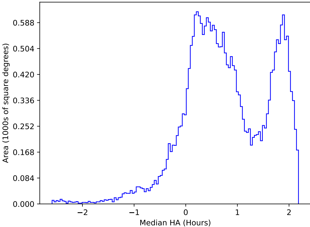
roll_pause_mjdp60_v3.4_10yrs All sky i band: Median HA
