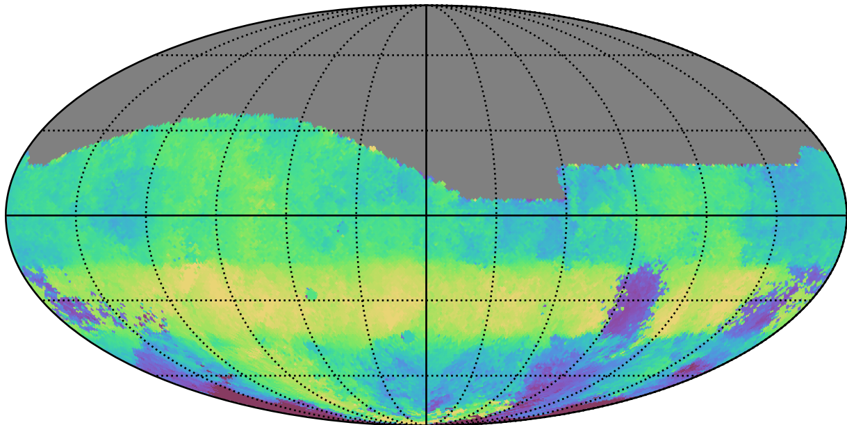
roll_pause_mjdp60_v3.4_10yrs All sky g band: Median HA
