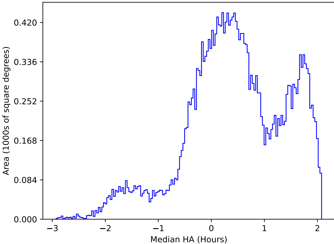
roll_pause_mjdp60_v3.4_10yrs All sky g band: Median HA
