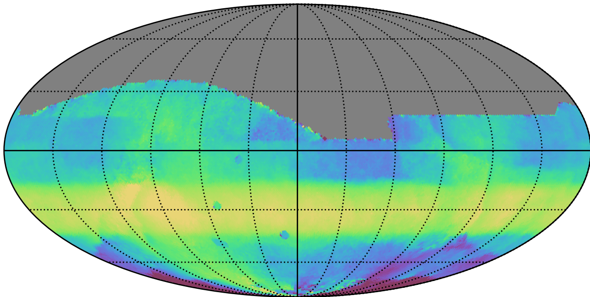
roll_pause_mjdp60_v3.4_10yrs All sky all bands: Median HA
