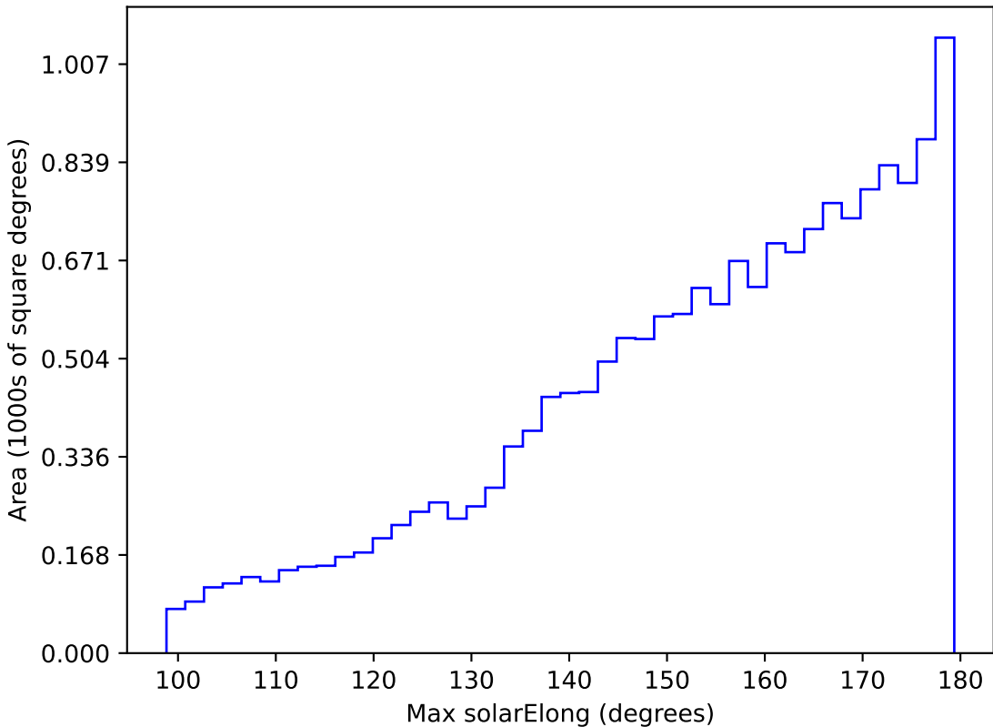
roll_pause_mjdp60_v3.4_10yrs WFD z band: Max solarElong
