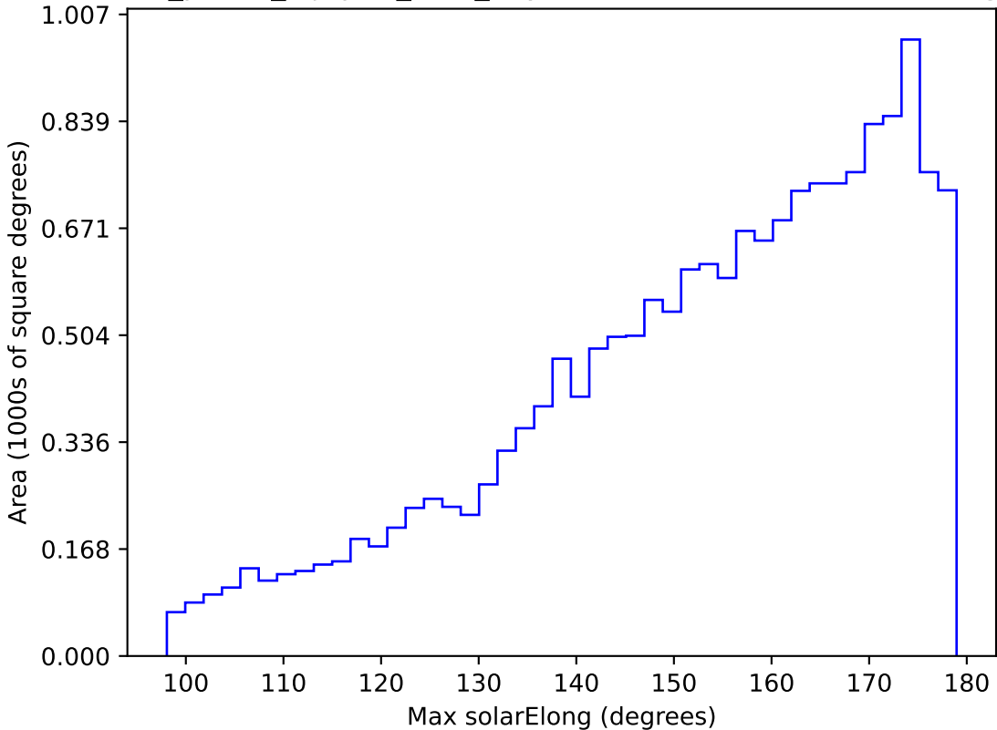
roll_pause_mjdp60_v3.4_10yrs WFD u band: Max solarElong
