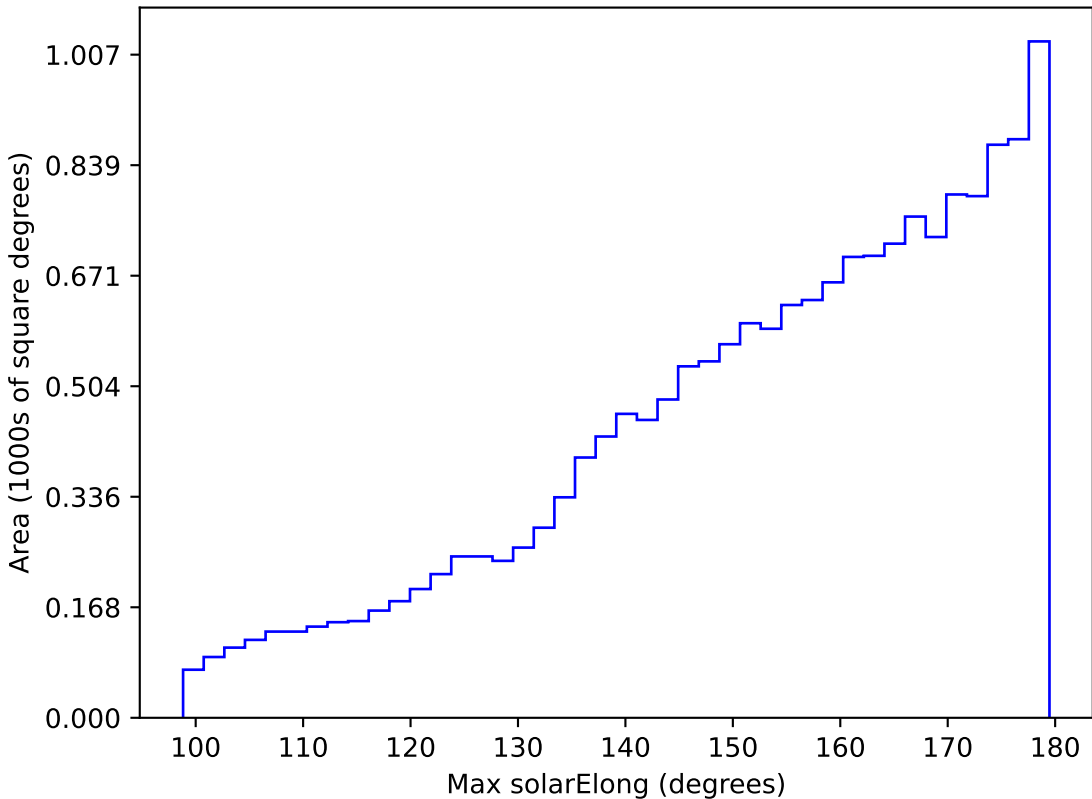
roll_pause_mjdp60_v3.4_10yrs WFD i band: Max solarElong
