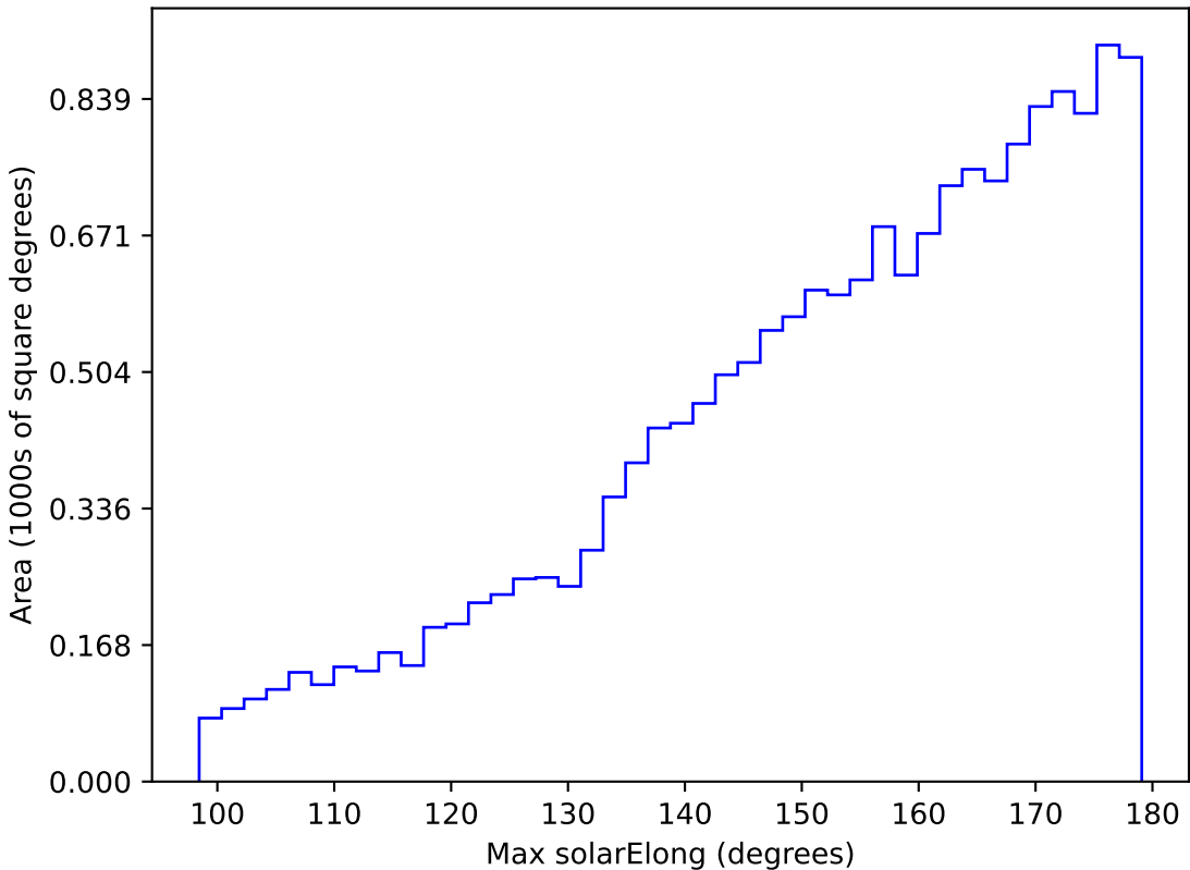
roll_pause_mjdp60_v3.4_10yrs WFD g band: Max solarElong
