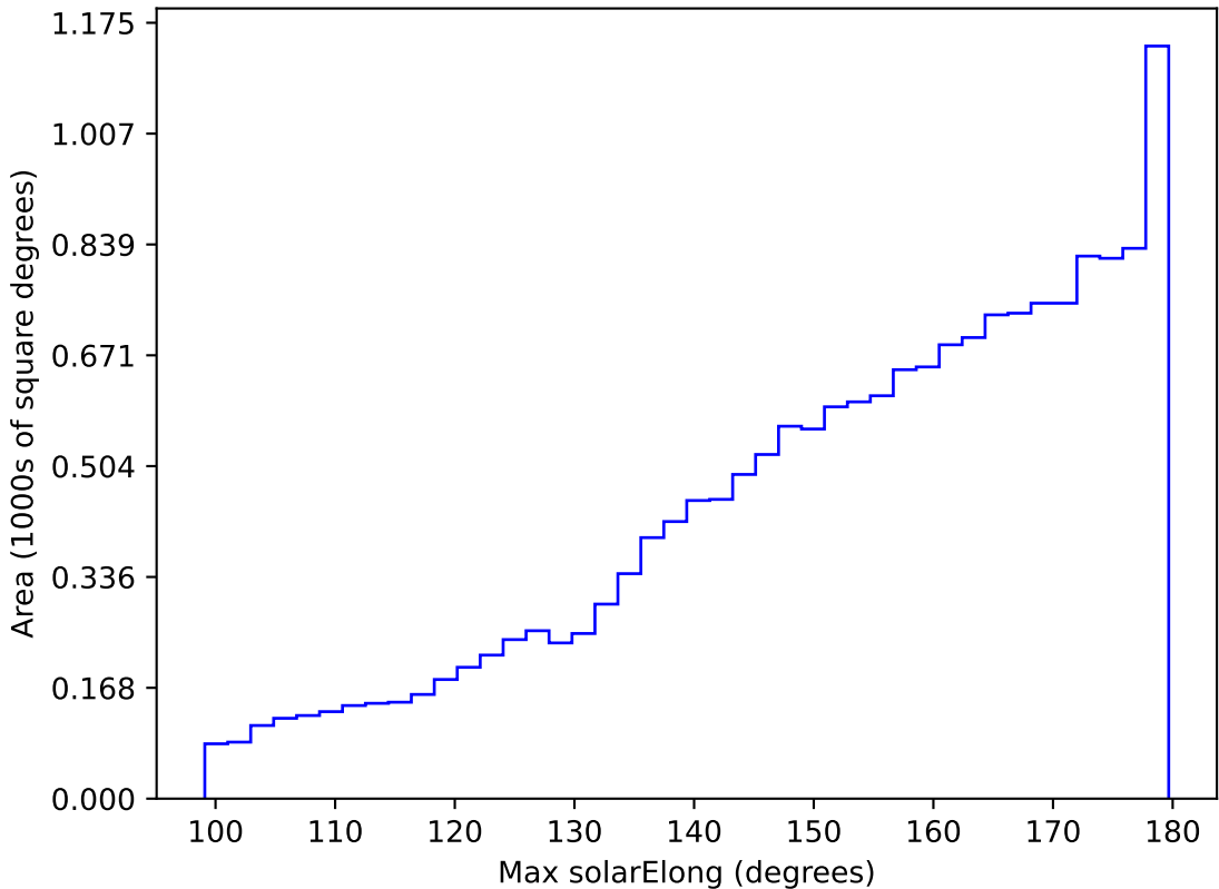
roll_pause_mjdp60_v3.4_10yrs WFD all bands: Max solarElong
