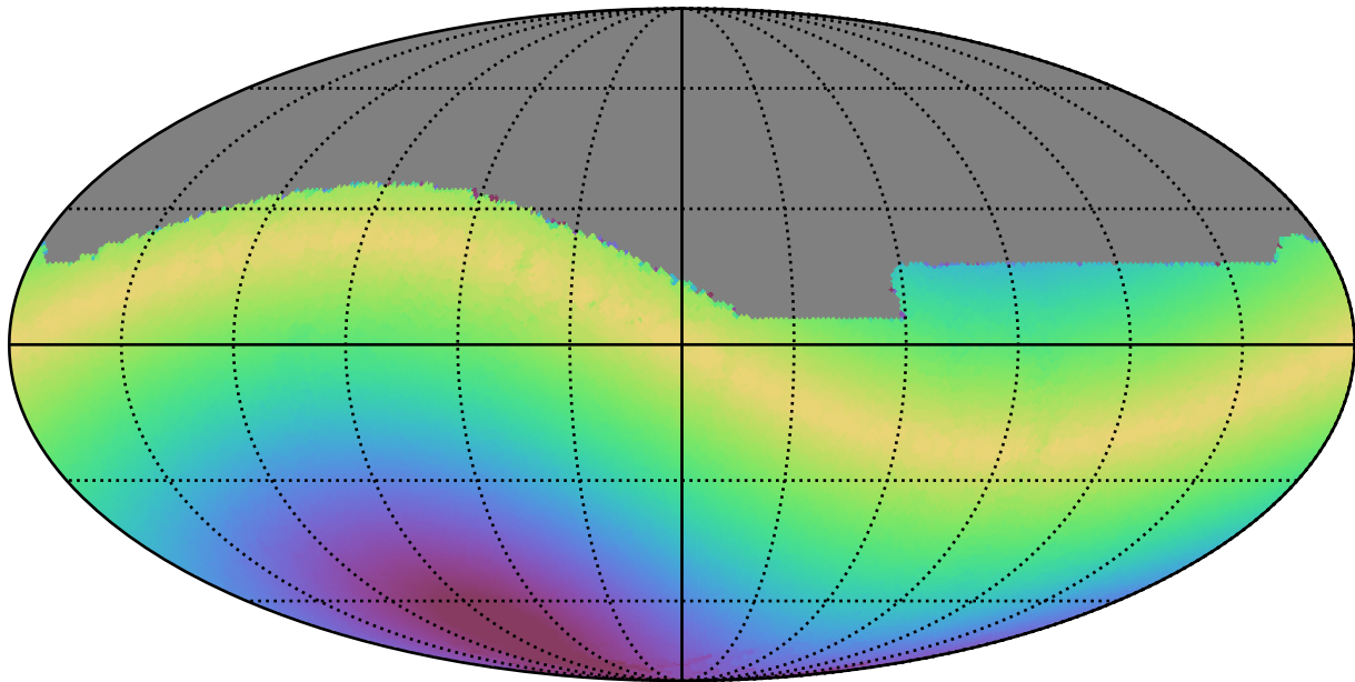
roll_pause_mjdp60_v3.4_10yrs All sky z band: Max solarElong
