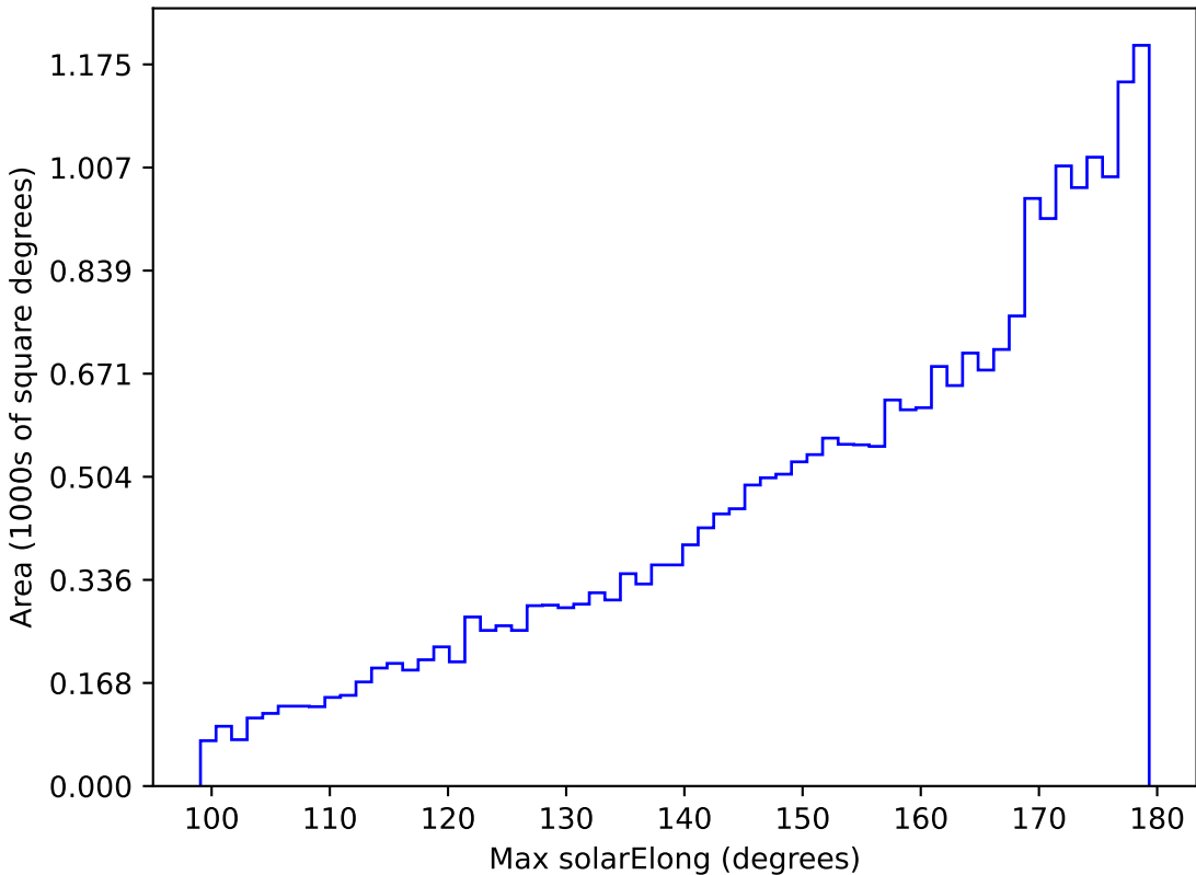
roll_pause_mjdp60_v3.4_10yrs All sky z band: Max solarElong
