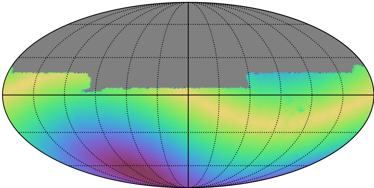
roll_pause_mjdp60_v3.4_10yrs All sky y band: Max solarElong
