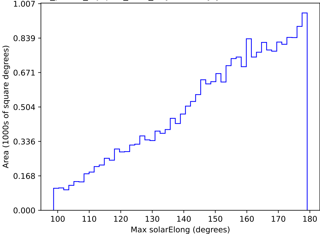
roll_pause_mjdp60_v3.4_10yrs All sky y band: Max solarElong
