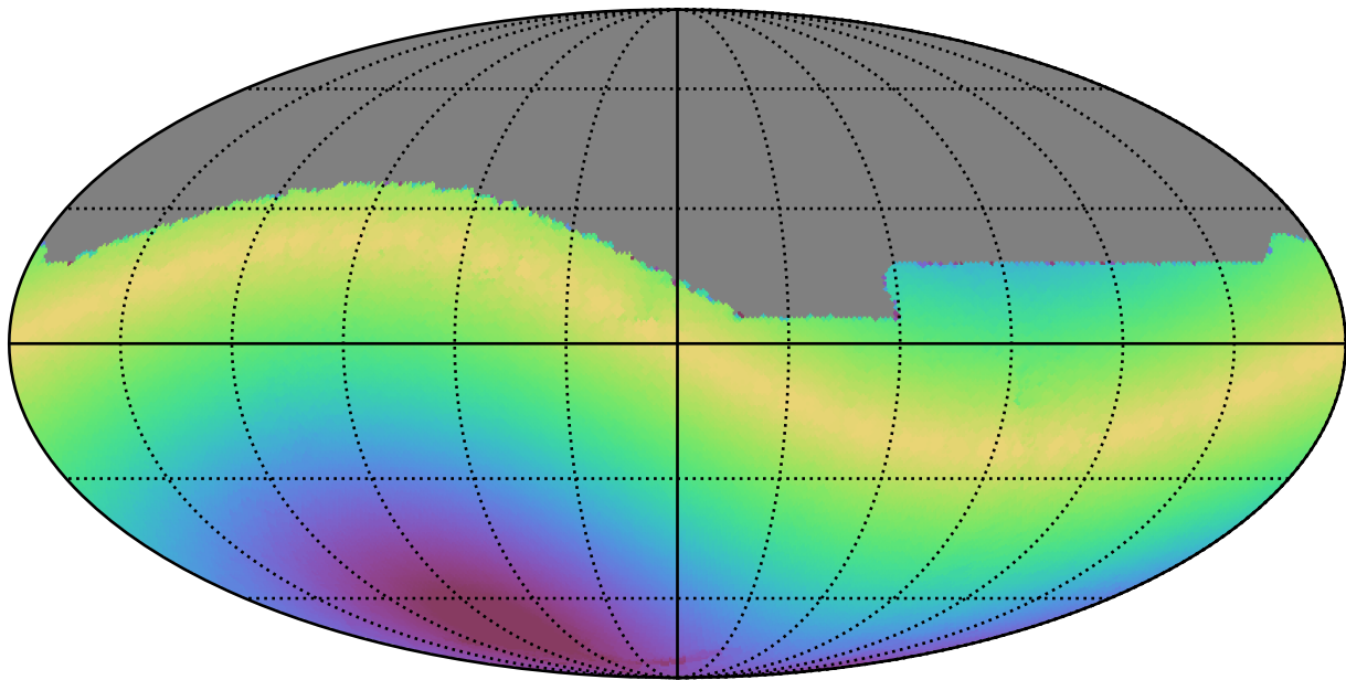
roll_pause_mjdp60_v3.4_10yrs All sky r band: Max solarElong
