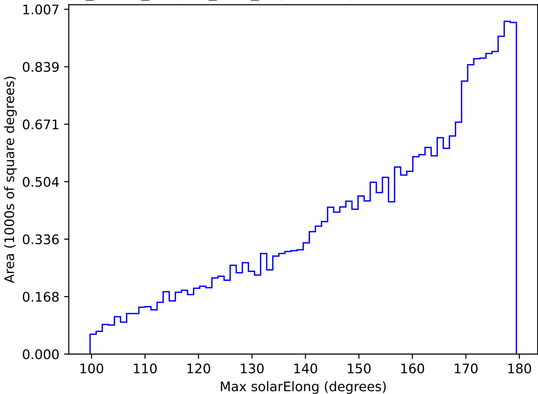
roll_pause_mjdp60_v3.4_10yrs All sky r band: Max solarElong
