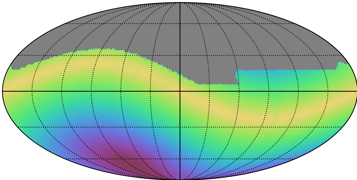
roll_pause_mjdp60_v3.4_10yrs All sky i band: Max solarElong
