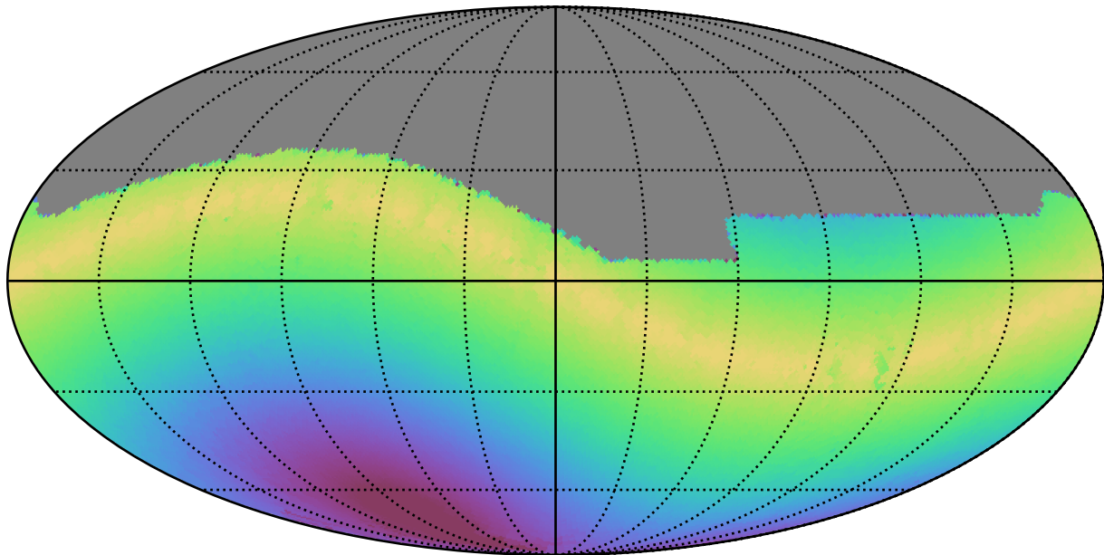
roll_pause_mjdp60_v3.4_10yrs All sky g band: Max solarElong
