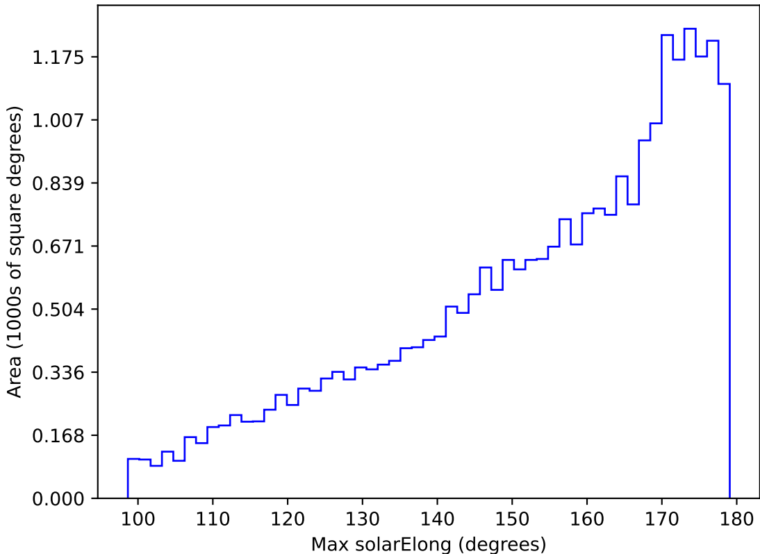
roll_pause_mjdp60_v3.4_10yrs All sky g band: Max solarElong
