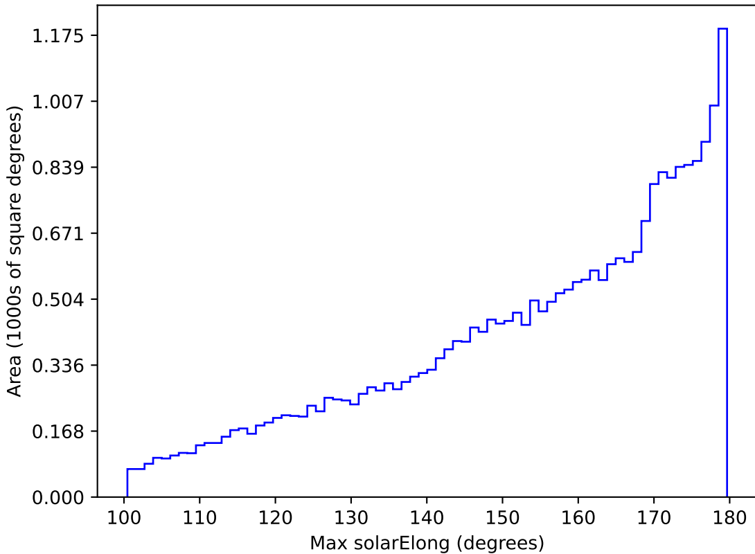
roll_pause_mjdp60_v3.4_10yrs All sky all bands: Max solarElong
