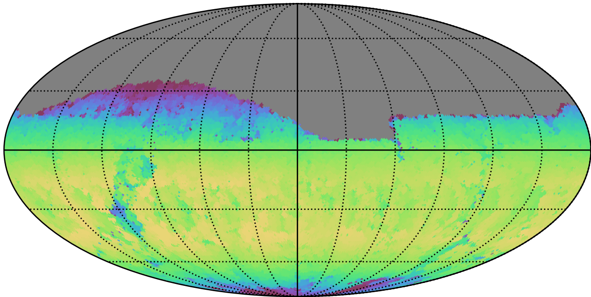
roll_pause_mjdp60_v3.4_10yrs Yr 1 z band: Max skyBrightness
