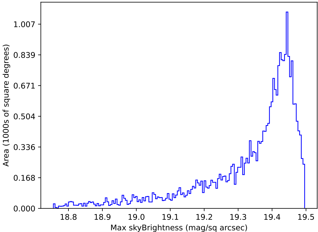
roll_pause_mjdp60_v3.4_10yrs Yr 1 z band: Max skyBrightness
