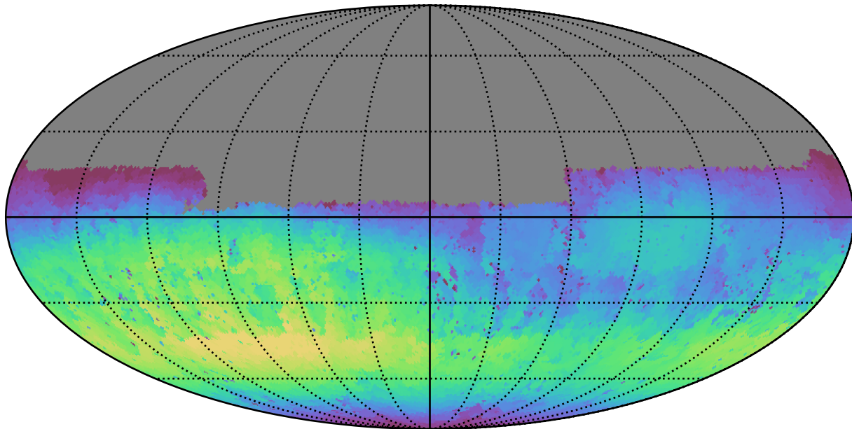
roll_pause_mjdp60_v3.4_10yrs Yr 1 u band: Max skyBrightness
