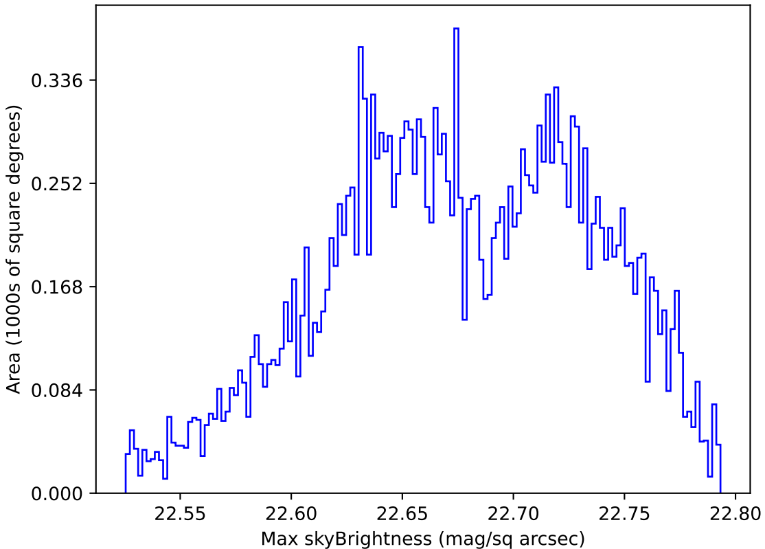
roll_pause_mjdp60_v3.4_10yrs Yr 1 u band: Max skyBrightness
