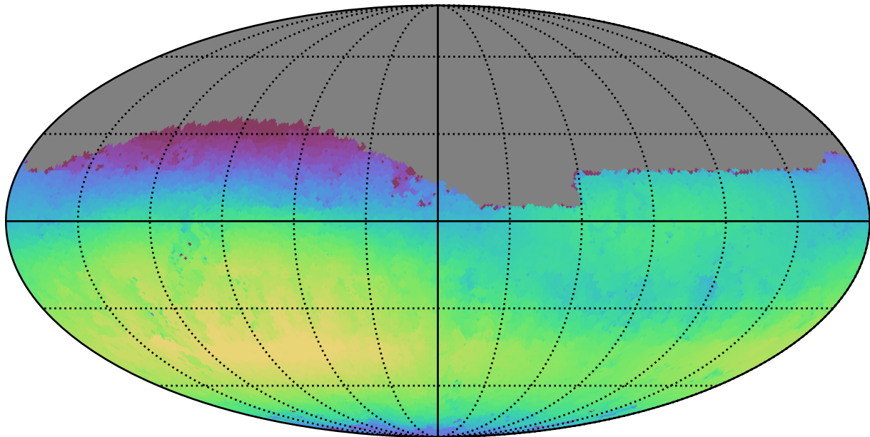
roll_pause_mjdp60_v3.4_10yrs Yr 1 r band: Max skyBrightness
