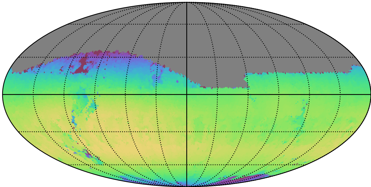
roll_pause_mjdp60_v3.4_10yrs Yr 1 i band: Max skyBrightness
