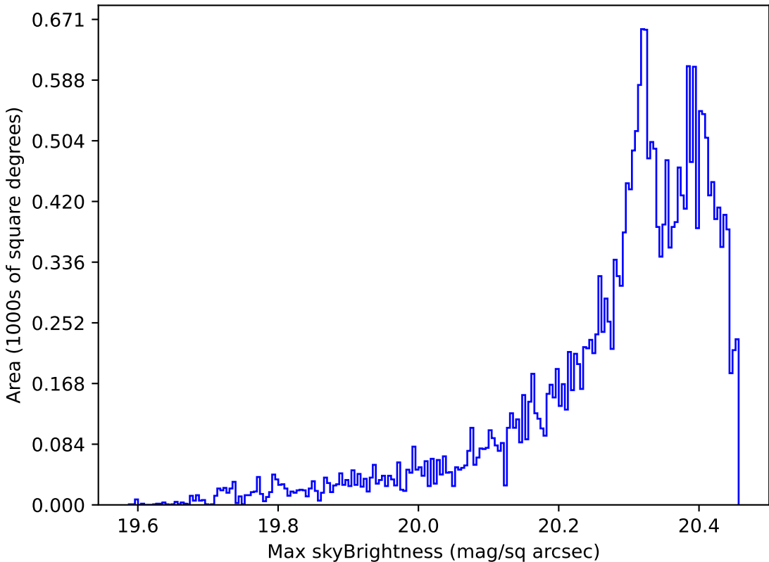
roll_pause_mjdp60_v3.4_10yrs Yr 1 i band: Max skyBrightness
