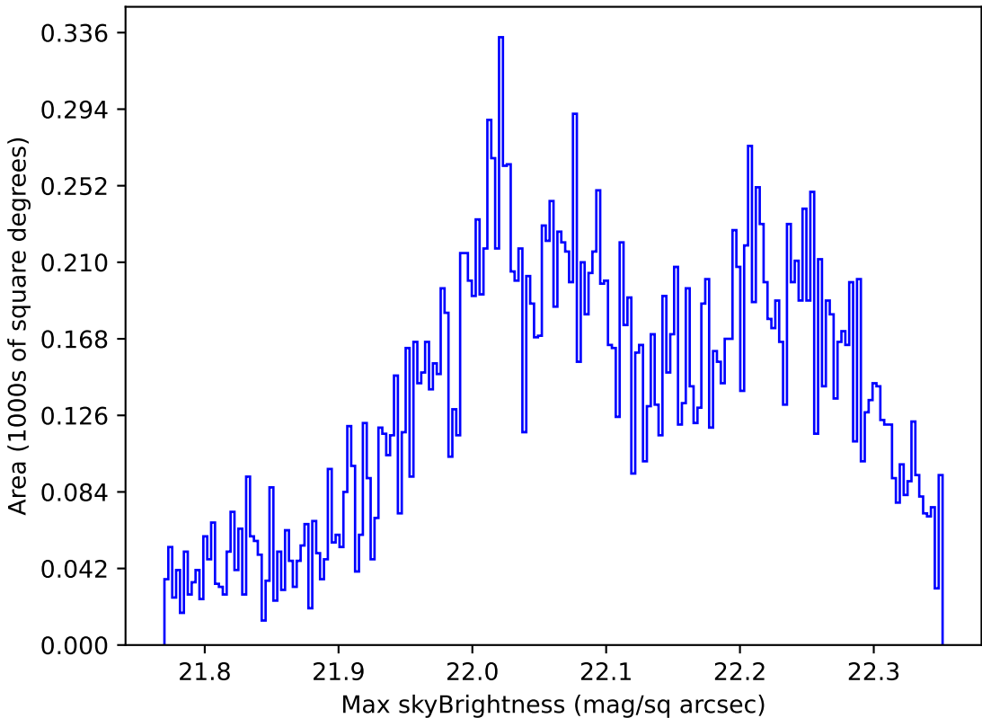
roll_pause_mjdp60_v3.4_10yrs Yr 1 g band: Max skyBrightness
