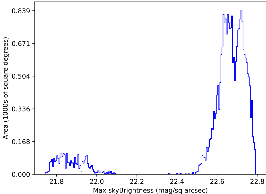
roll_pause_mjdp60_v3.4_10yrs Yr 1 all bands: Max skyBrightness
