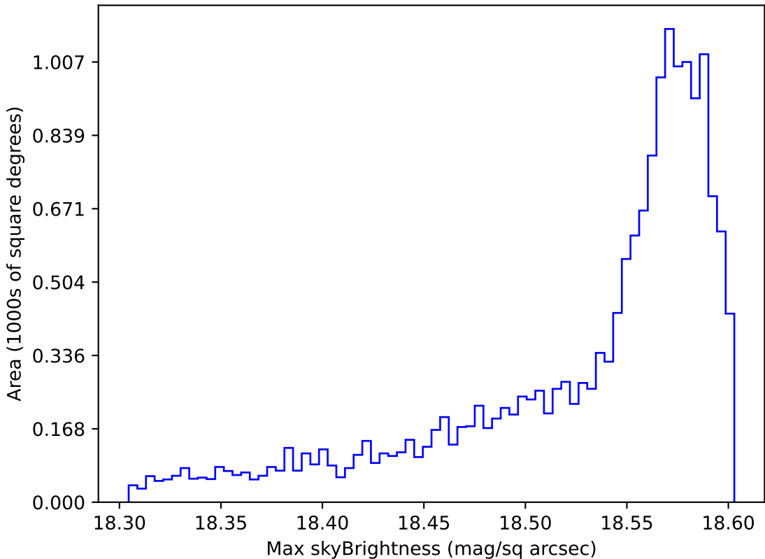
roll_pause_mjdp60_v3.4_10yrs WFD y band: Max skyBrightness
