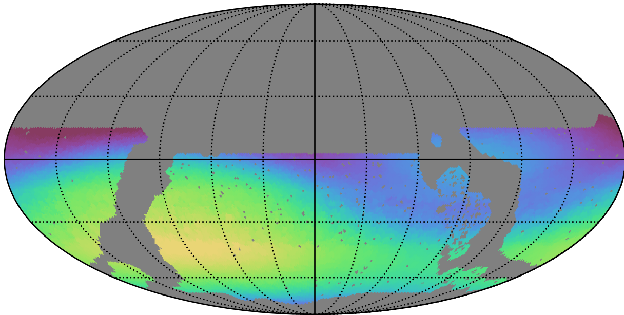
roll_pause_mjdp60_v3.4_10yrs WFD r band: Max skyBrightness
