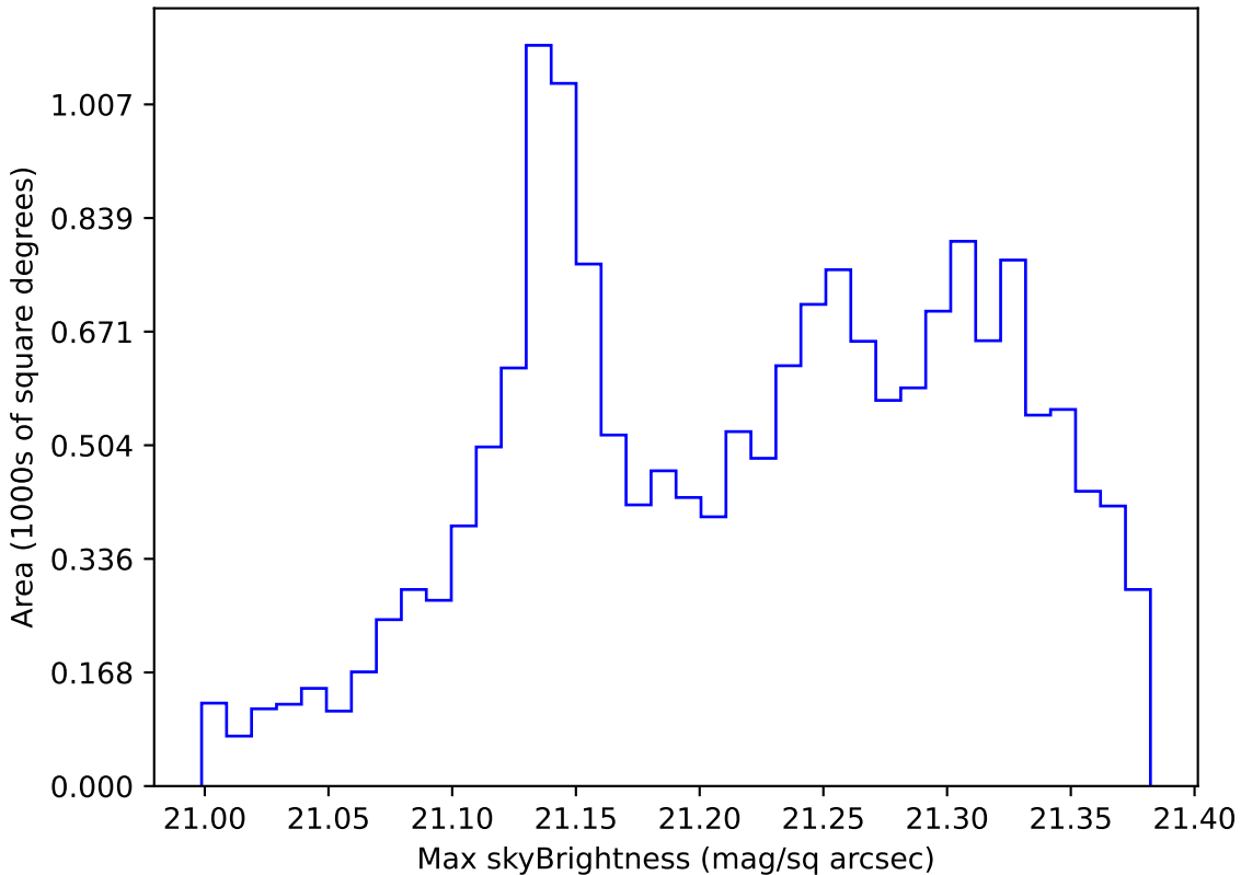
roll_pause_mjdp60_v3.4_10yrs WFD r band: Max skyBrightness
