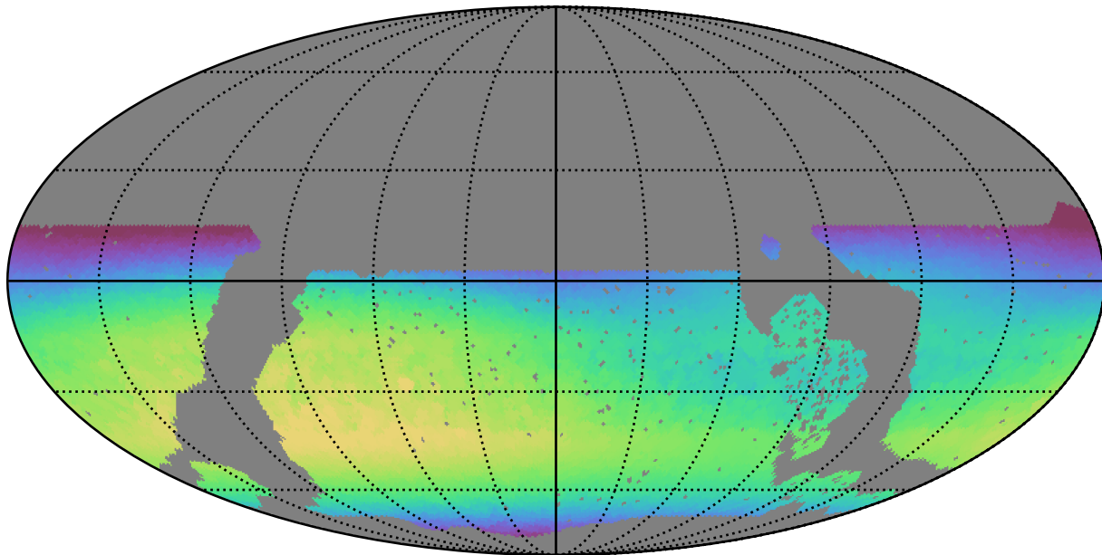
roll_pause_mjdp60_v3.4_10yrs WFD i band: Max skyBrightness
