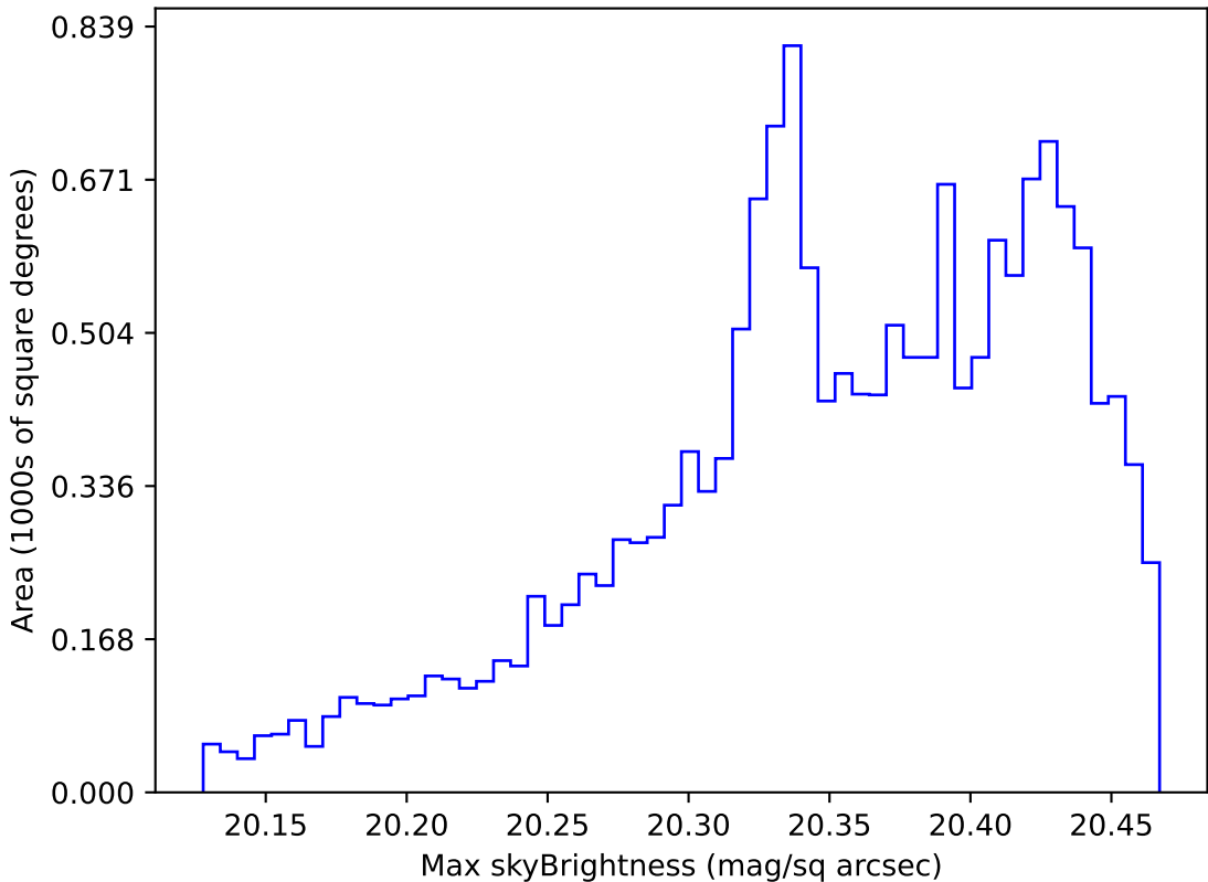
roll_pause_mjdp60_v3.4_10yrs WFD i band: Max skyBrightness
