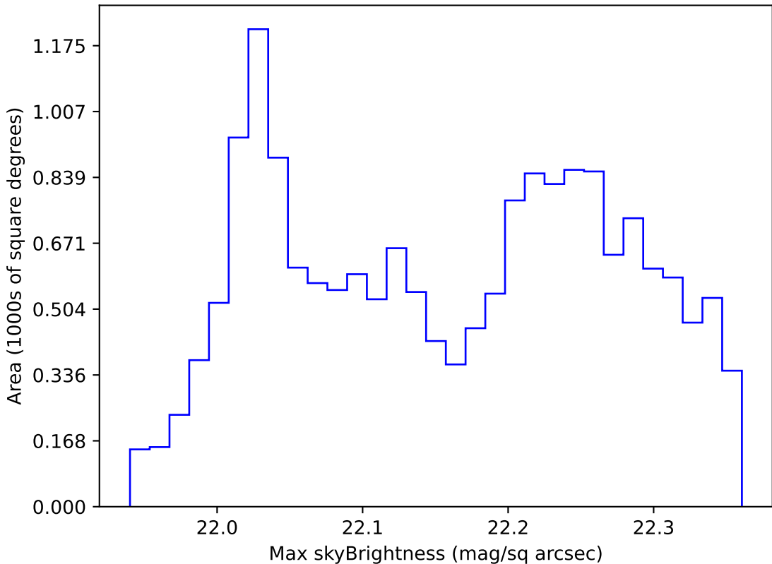
roll_pause_mjdp60_v3.4_10yrs WFD g band: Max skyBrightness
