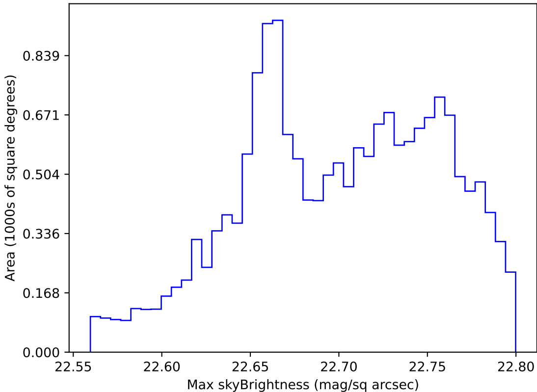
roll_pause_mjdp60_v3.4_10yrs WFD all bands: Max skyBrightness
