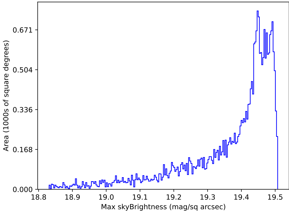
roll_pause_mjdp60_v3.4_10yrs All sky z band: Max skyBrightness
