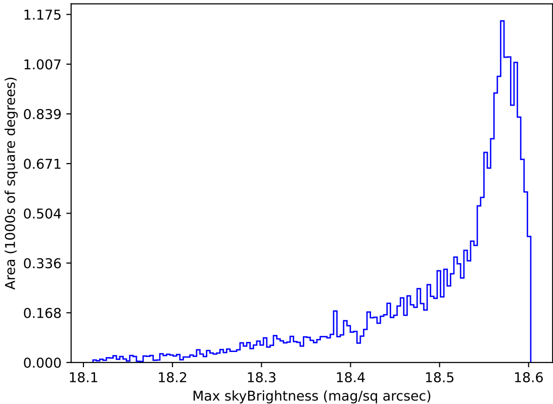
roll_pause_mjdp60_v3.4_10yrs All sky y band: Max skyBrightness
