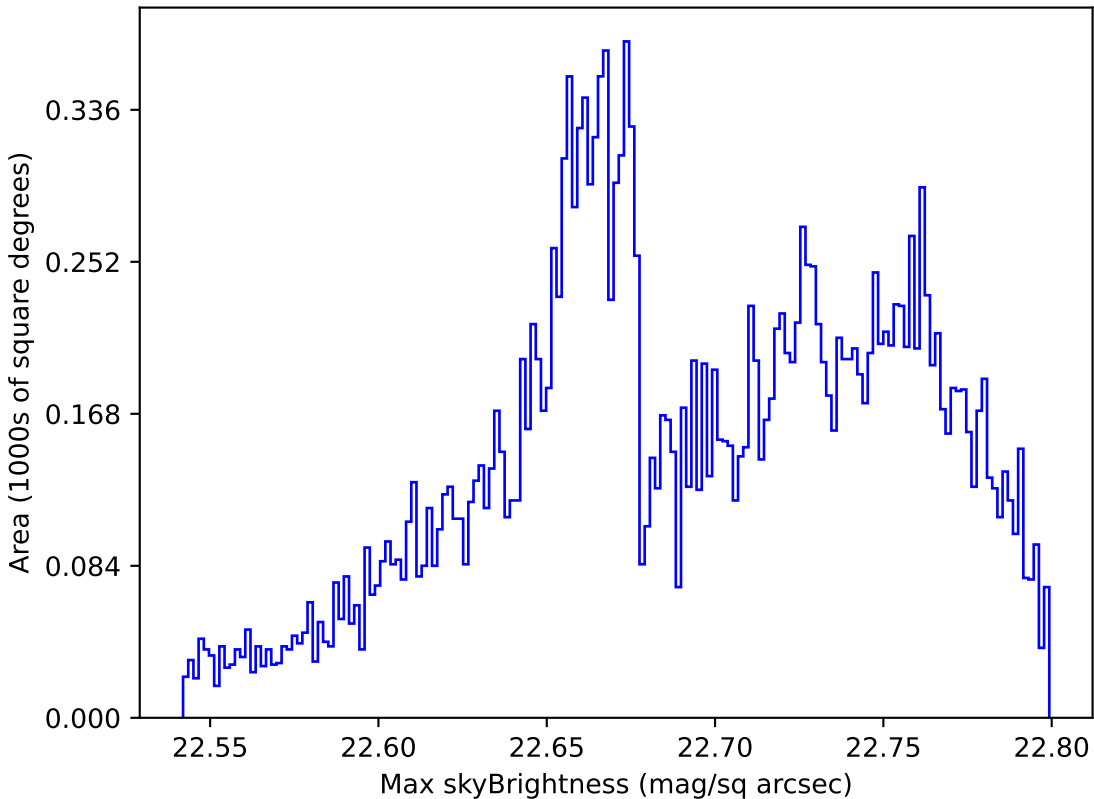
roll_pause_mjdp60_v3.4_10yrs All sky u band: Max skyBrightness
