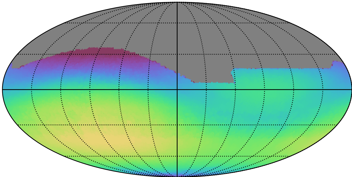
roll_pause_mjdp60_v3.4_10yrs All sky r band: Max skyBrightness
