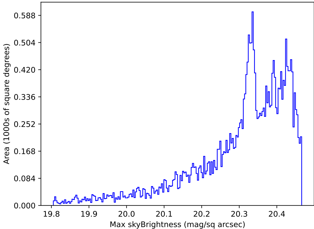
roll_pause_mjdp60_v3.4_10yrs All sky i band: Max skyBrightness
