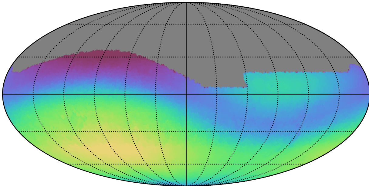
roll_pause_mjdp60_v3.4_10yrs All sky g band: Max skyBrightness
