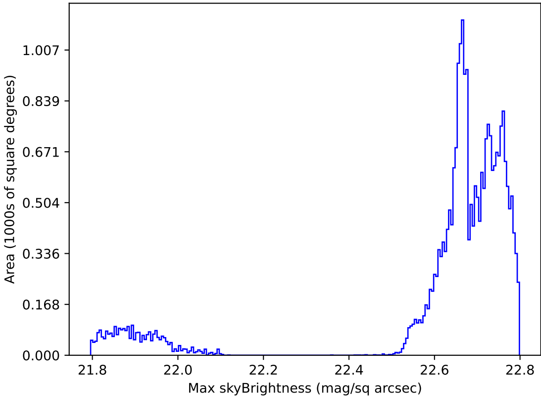
roll_pause_mjdp60_v3.4_10yrs All sky all bands: Max skyBrightness
