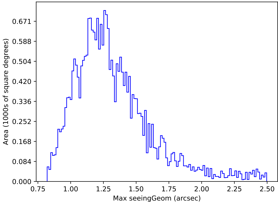
roll_pause_mjdp60_v3.4_10yrs Yr 1 z band: Max seeingGeom
