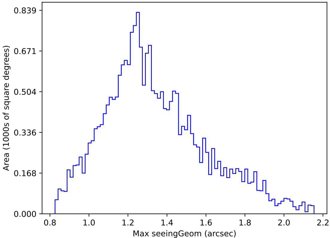
roll_pause_mjdp60_v3.4_10yrs Yr 1 u band: Max seeingGeom
